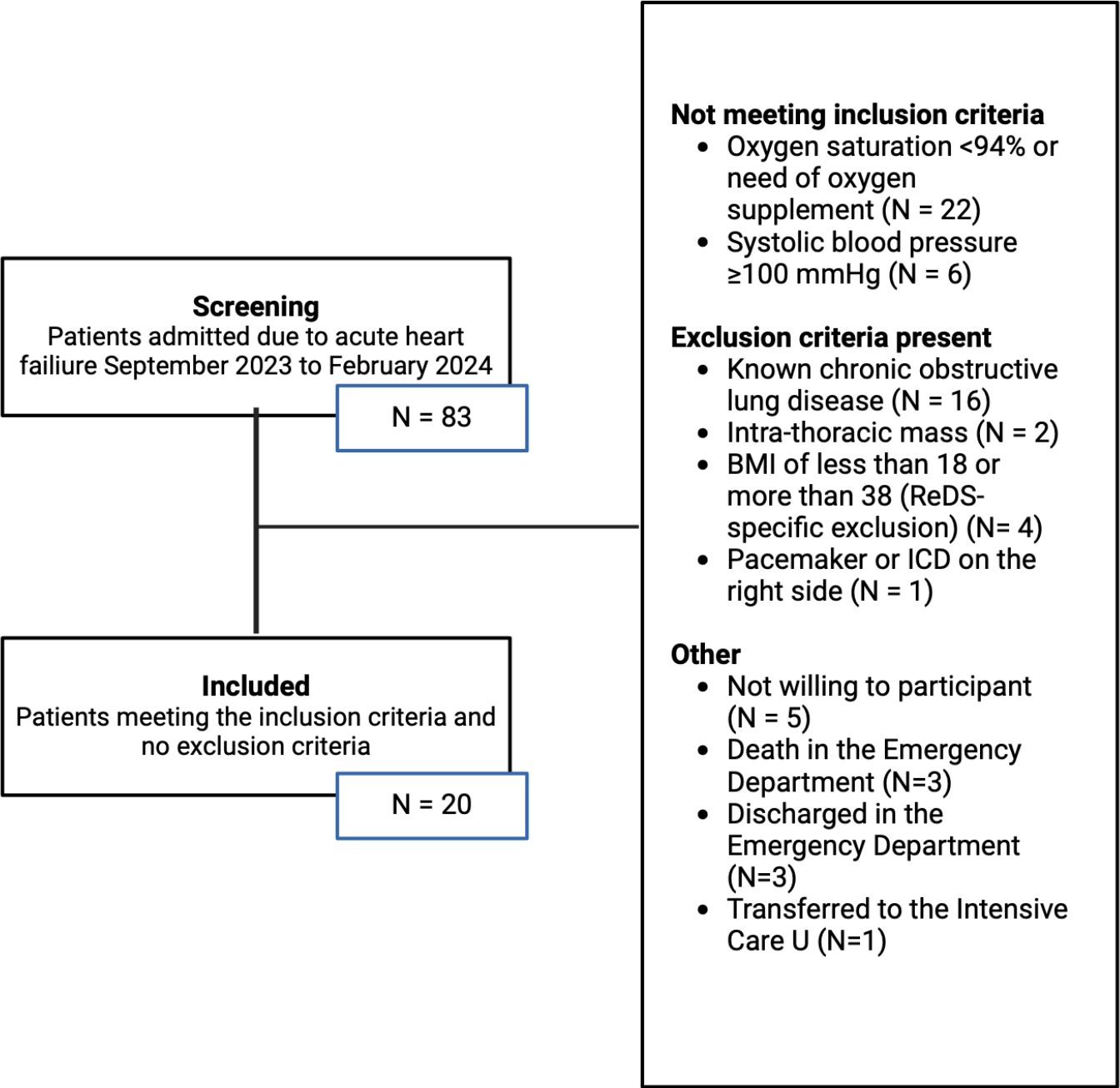
Figure 2: Study flowchart
