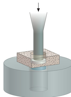
Figure 11. Mechanical testing. Axial push out test with specimen placed on metal platform with central opening. Specimen thickness nominal 3.5 mm, implant nominal diameter 6 mm, support hole diameter 7.4 mm, preload 2N, displacement velocity 5 mm/min.
