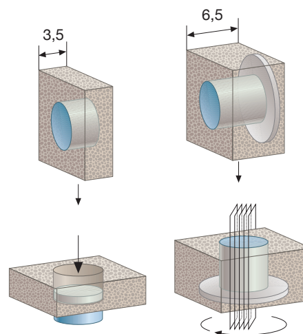
Figure 5. Sectioning technique illustrated with specimen from study III. Left image: outer section specimen (3.5 mm) for mechanical testing. Right image: Inner section specimen (6.5 mm) for histomorphometry using the vertical section method applying 4 sections around implant centre after random rotation around implant axis.
