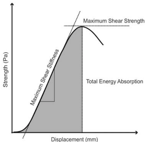
Figure 12. Mechanical testing. Normalisation of load-displacement curve enables calculation of maximum shear strength (MPa), maximum shear stiffness (MPa/mm), total energy absorption (J/m 2 ).
