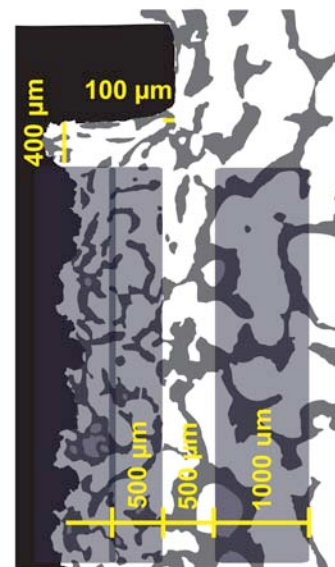
Figure 7. Study II. Gap. Histomorphometry. Schematic drawing. Region of interest (ROI) collectively defined on both implant sides, but illustrated on one side above: a) tissue ongrowth (surface fraction) at interface, b) tissue volume fraction in gap divided in two of an inner gap region and an outer gap region (500 \mu\text{m} ), and c) tissue volume fraction in region of intact non-implanted bone (1000 \mu\text{m} ). Regions defined from washer margin as a fixed point with a 100 \mu\text{m} clearance at gap-intact-bone-interface and 400 \mu\text{m} below washer.
