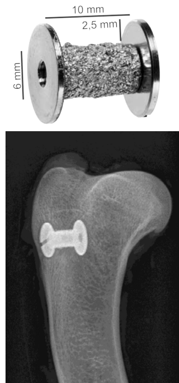
Figure 3. Study III. Allografted gap implant model. Gap implant device, dimension 10x6 mm surrounded by a 2.5 mm gap impacted with morsellised allograft bone secured by 11 mm washer. Implant in host of cancellous bone in the right proximal humerus. X-ray image at time of bone harvest completing 4 weeks treatment of PTH/control.
