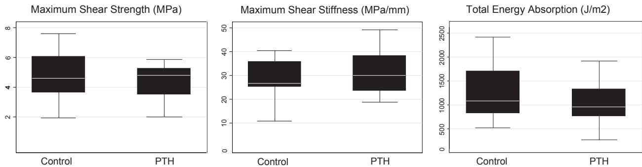
Figure 18: Study III. Graft. Mechanical results. Box plot. Maximum shear strength, maximum shear stiffness, and total energy absorption. n(\text{control}) = 9 , n(\text{PTH}) = 8 . Mann-Whitney test. No significant ( p \geq 0.05 ) differences PTH compared to control.
