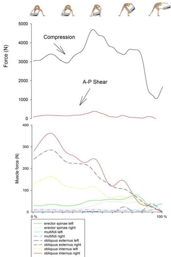
Figure 8 Stooped task. The time course of compression and A/P shear forces are on top and corresponding muscle forces are below
